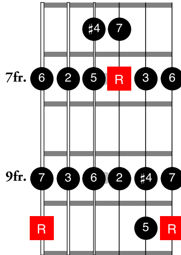
D Lydian
