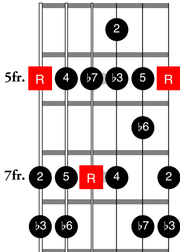
A Aeolian
