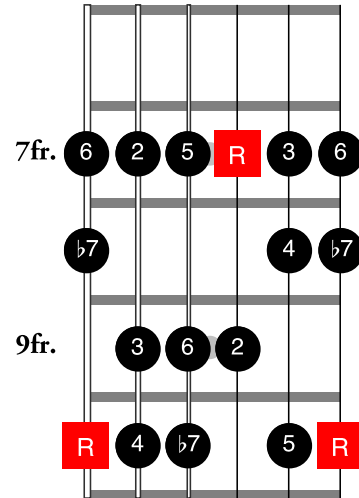
D Mixolydian
