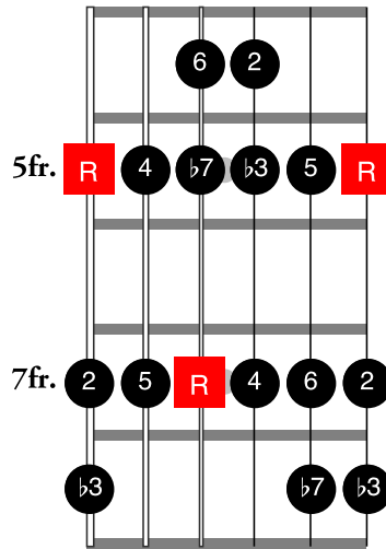
A Dorian
